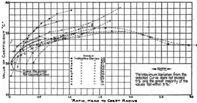
FIG. 15.—Diagram showing relation of "C" values to the ratio of head to crest radius. Experiments on curve crested dams.
